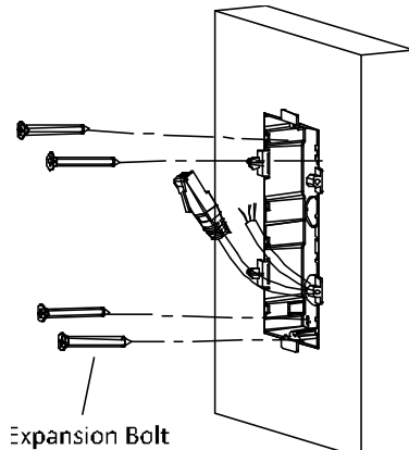
Figure 3-29 Fix the Gang Box
